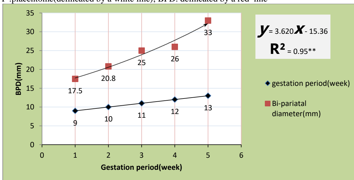
Fig.4-Relationships between the biparietal diameter (BPD), and the gestational age (GA), y = BPD(mm), x = gestational age, R^2 = squares of correlation coefficient
